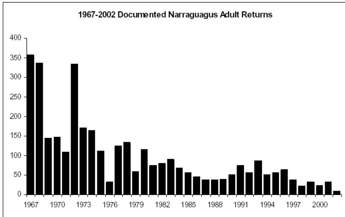
Figure 6.4.18: Upper panel: Estimated returns of adult Atlantic salmon to rivers of the Distinct Population Segment, 1991-2002. Lower panel: Documented returns of adult Atlantic salmon to the Narraguagus River, 1967-2002. (Figures from NMFS/USFWS 2004.)
