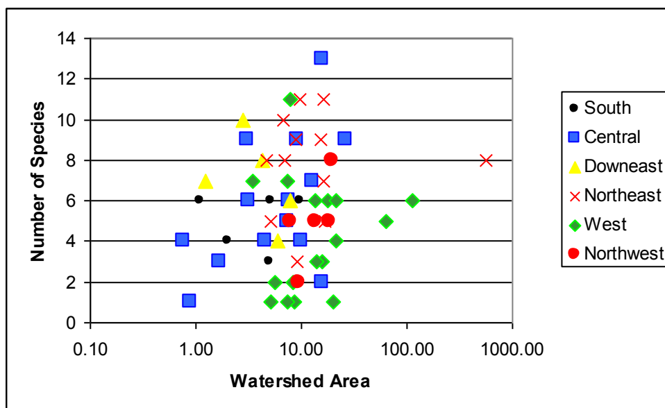
Figure 6.4.6: Species richness in stream fish assemblages, as a function of stream size (watershed area, square miles).
