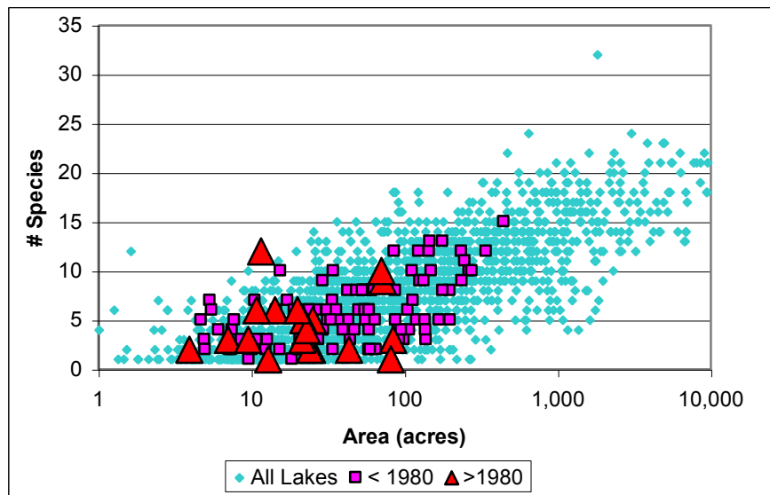
Figure 6.4.16: Fish species richness in reclaimed lakes as a function of lake area, compared to all lakes statewide.
